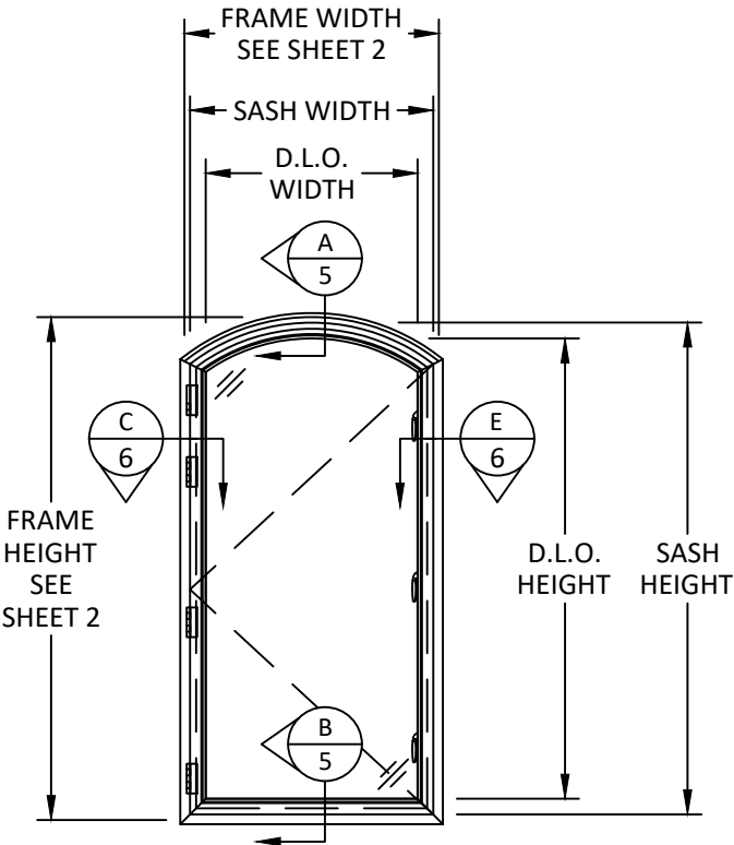
TYPICAL ELEVATION SINGLE CASEMENT, ARCH TOP
