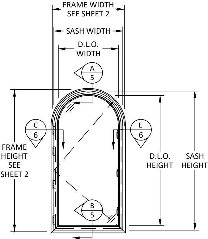
TYPICAL ELEVATION SINGLE CASEMENT, ROUND TOP
